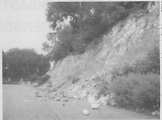
Figure 37 - Landslide. San Simeon Earthquake, December 22, 2003 Landslides on San Gregorio Road in Atascadero, California, only a short distance away from where the homes with the most damage were located.
