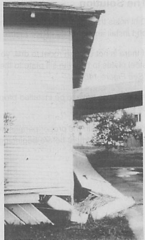
Figure 15 - Damage to home due to cripple wall failure.
