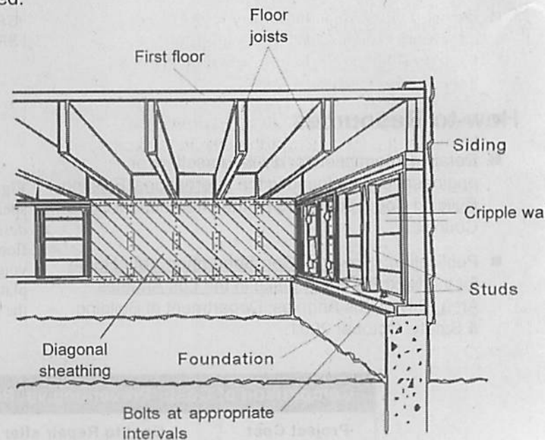
Figure 16 - Diagonal Sheathing. Common in older homes.
