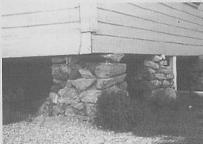
Figure 19 - This is an unreinforced stone foundation. They typically fail during earthquakes.
