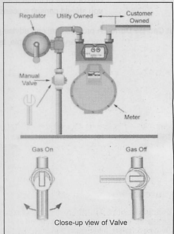
Figure 36—Manual Shutoff Valve Location
