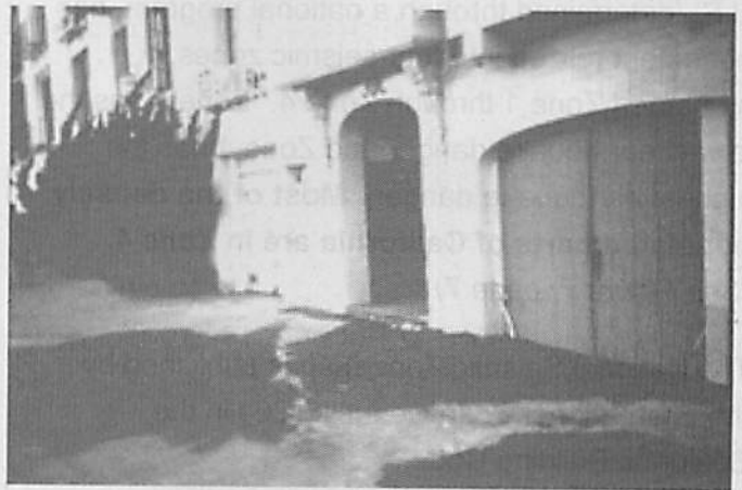
Figure 40 - Loma Prieta Earthquake, October 17, 1989. Lateral spreading, liquefaction and sand boils caused extensive damage in the Marina District of San Francisco, about 60 miles away from the epicenter.
